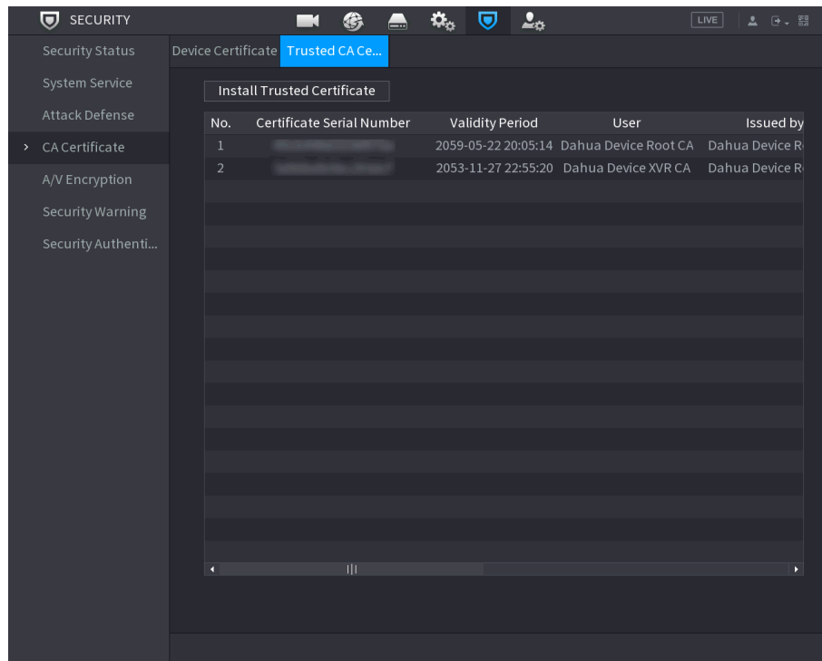
Figure 5-316 Trusted CA certificate
