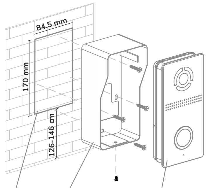
Niche Surface Bracket with Sun & Rain Cover Outdoor Panel
