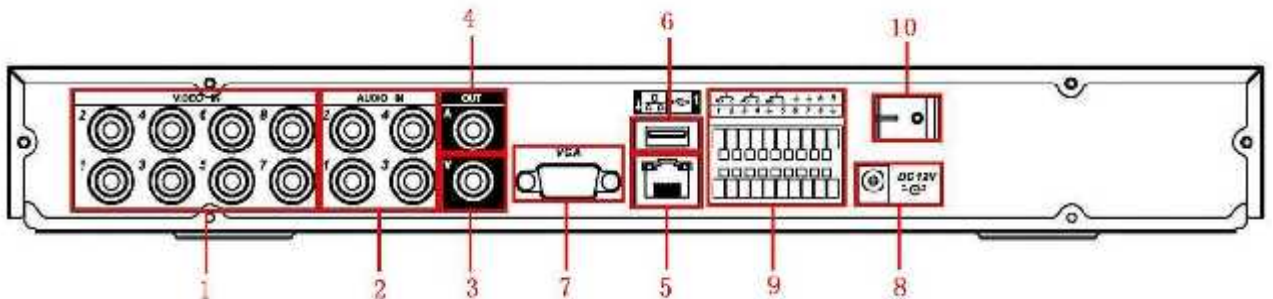
Figure 1-7 8-channel
