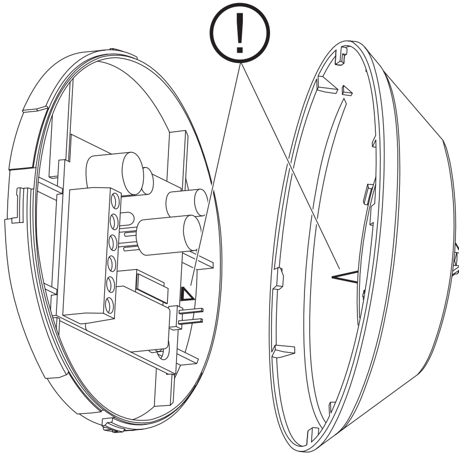
Fig. 3. Alignment of the matchmarks when closing the detector housing.
